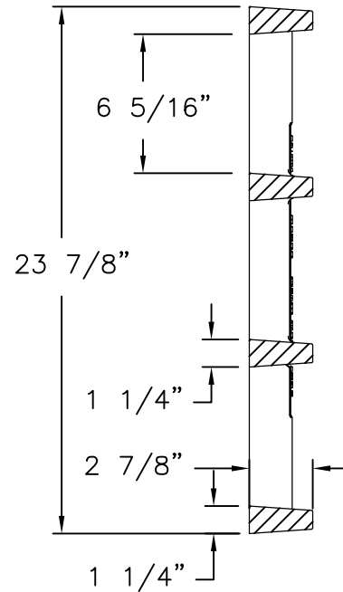
GRATE SECTION
